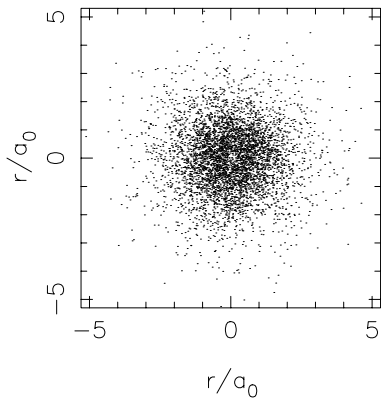
\psi_{211}
