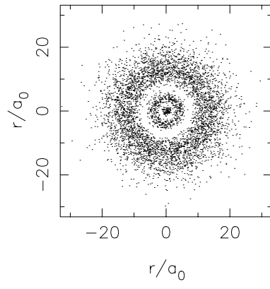
\psi_{320}
