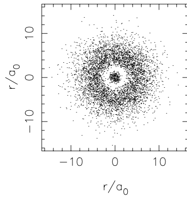
\psi_{300}
