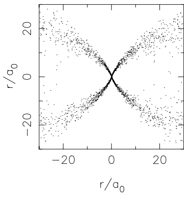
\psi_{322}
