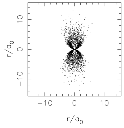
\psi_{310}
