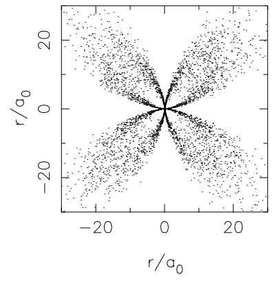
\psi_{410}
